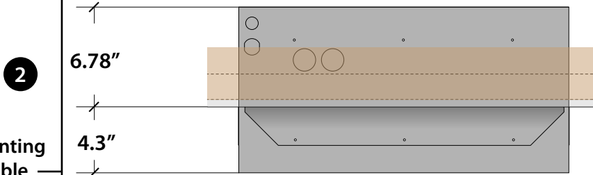
Partially Recessed Mounting Option
