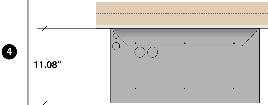
Fully Exposed Mounting Option
