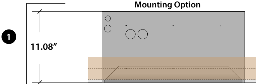
Partially Recessed Mounting Option
